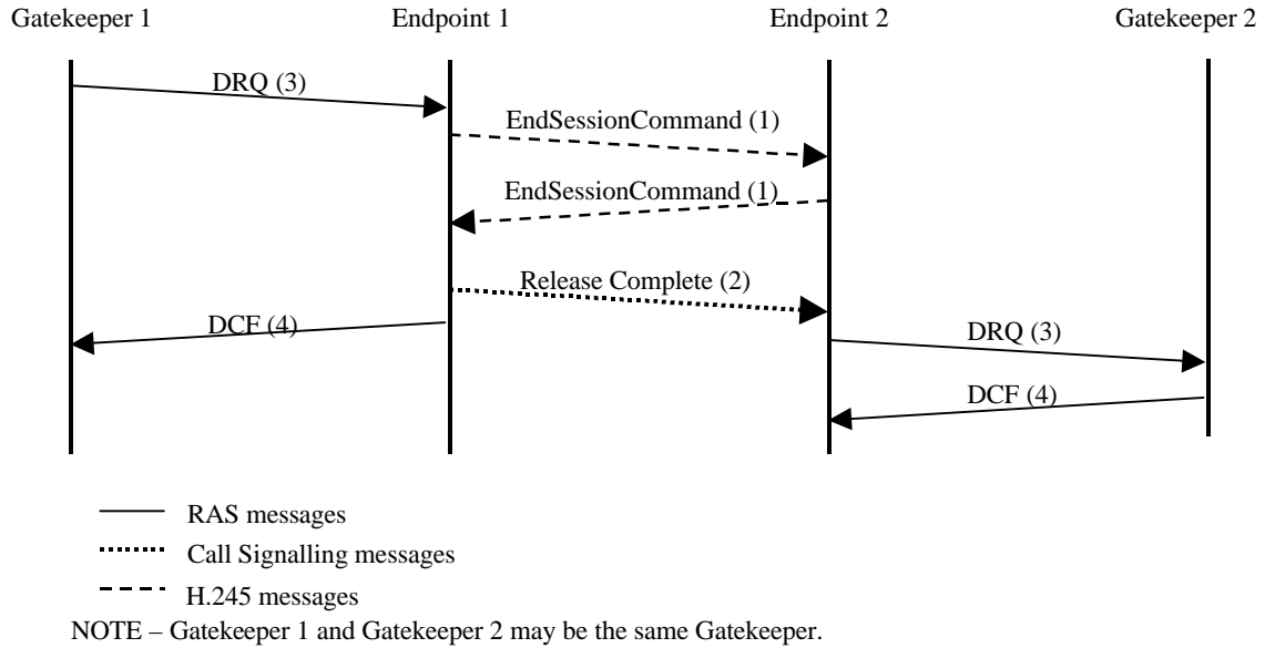
Figure 11 - Gatekeeper initiated call clearing
