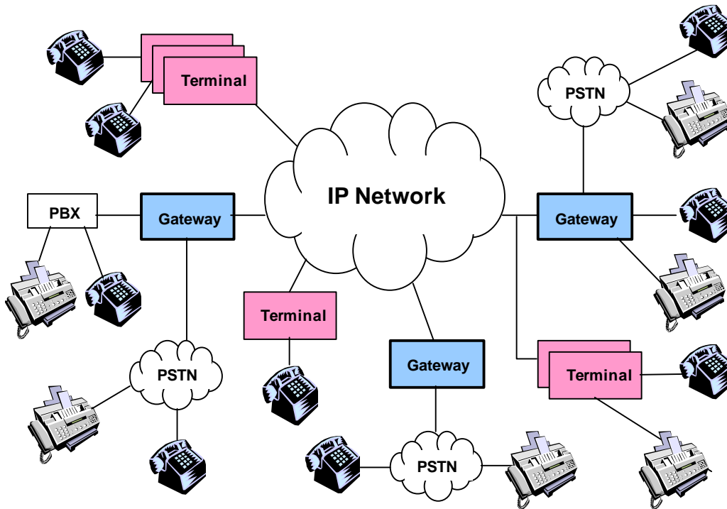
Figure 3 - Gateway interfacing with different networks
