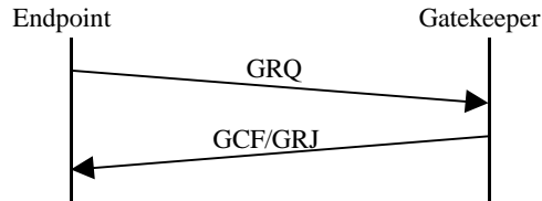
Figure 5 - Gatekeeper autodiscovery
