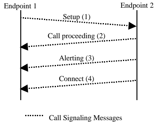
Figure 8 - Basic call setup, no Gatekeepers
