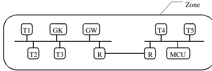
Figure 2 - H.323 zone
