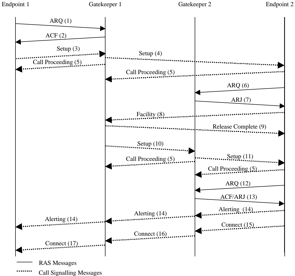
Figure 9 - Both endpoints registered, both gatekeepers routing call signaling
