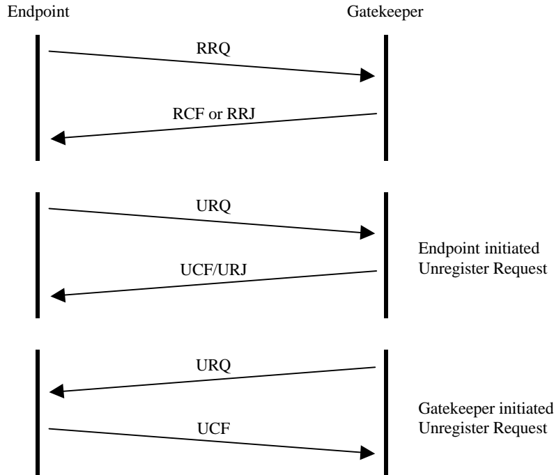
Figure 6 - Endpoint registration
