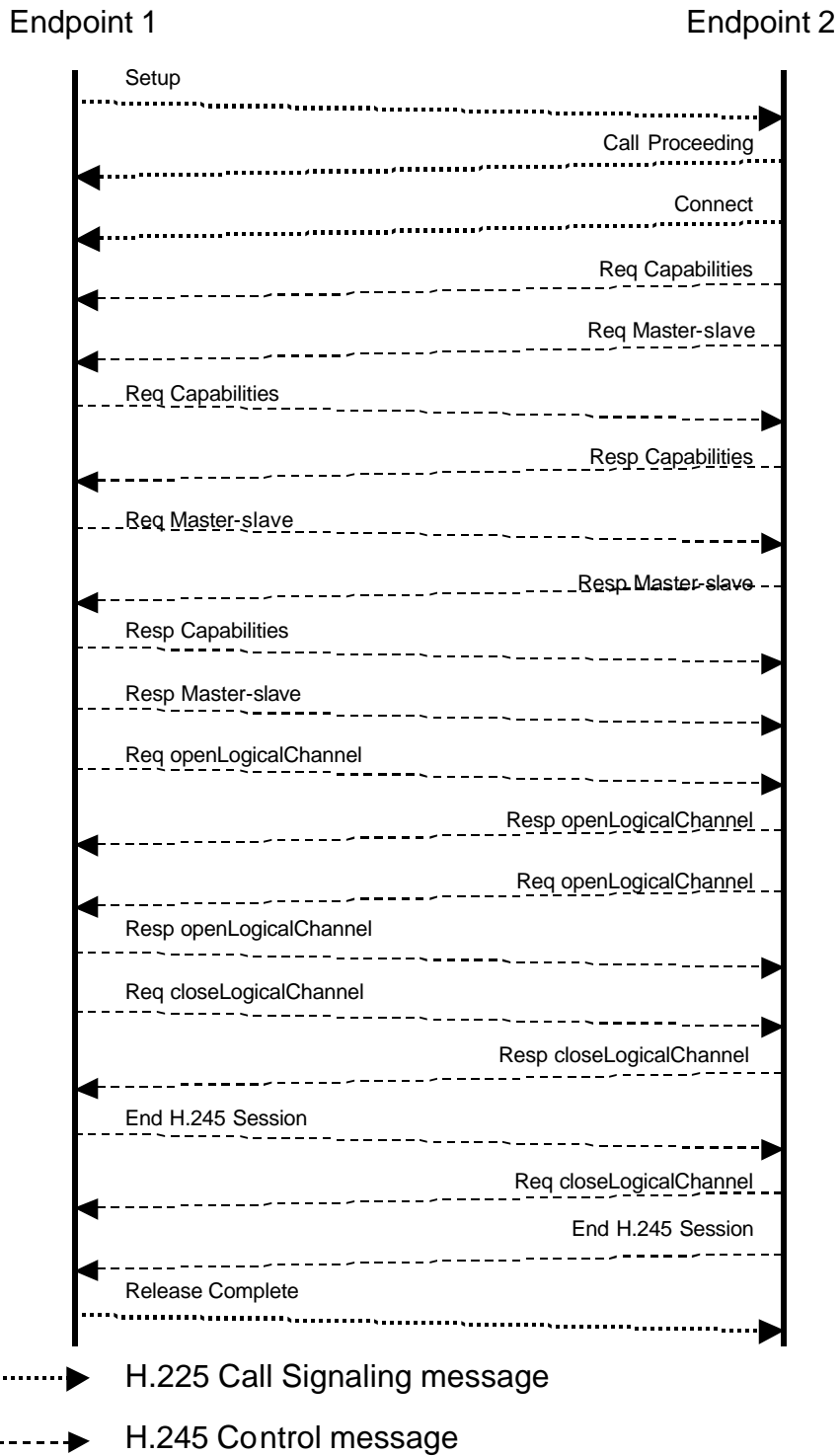
Figure 12 - Complete call signaling sequence
