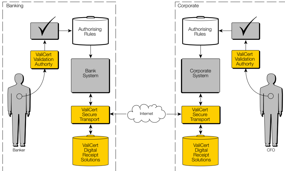
Bank-Corporate Treasury Management Solution Architecture
