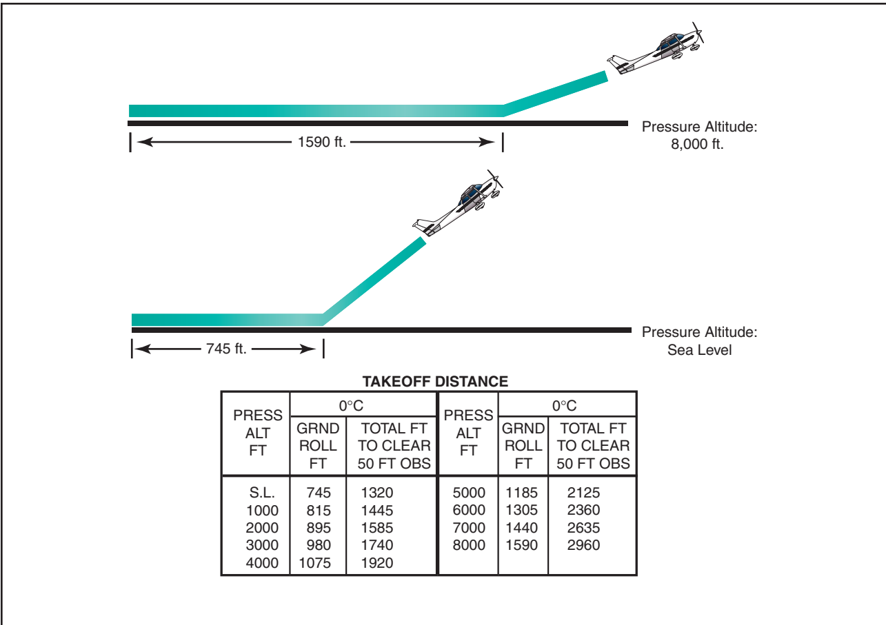
Figure 10-7. Takeoff distance increases with increased altitude.
