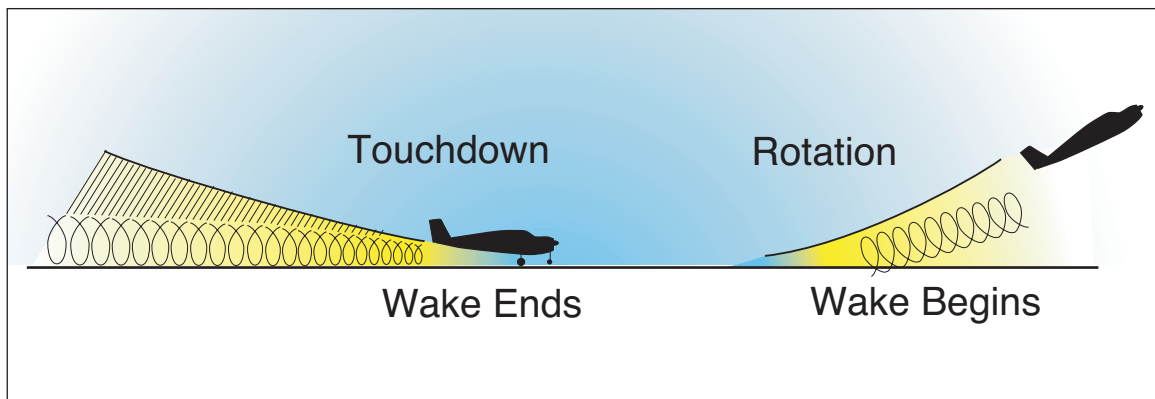
Figure 12-18. Vortex behavior.
