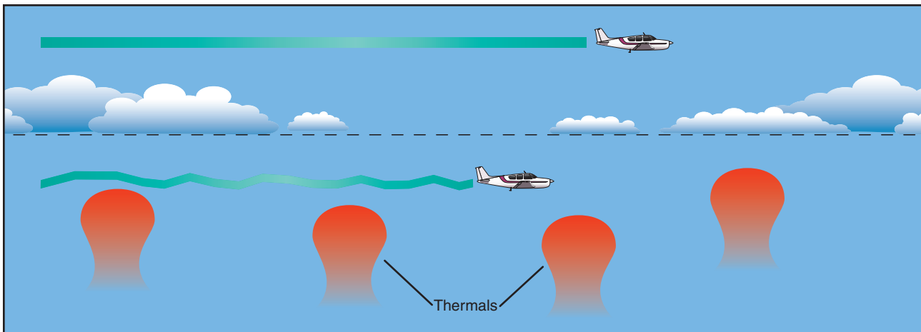
Figure 10-12. Convective turbulence avoidance.
