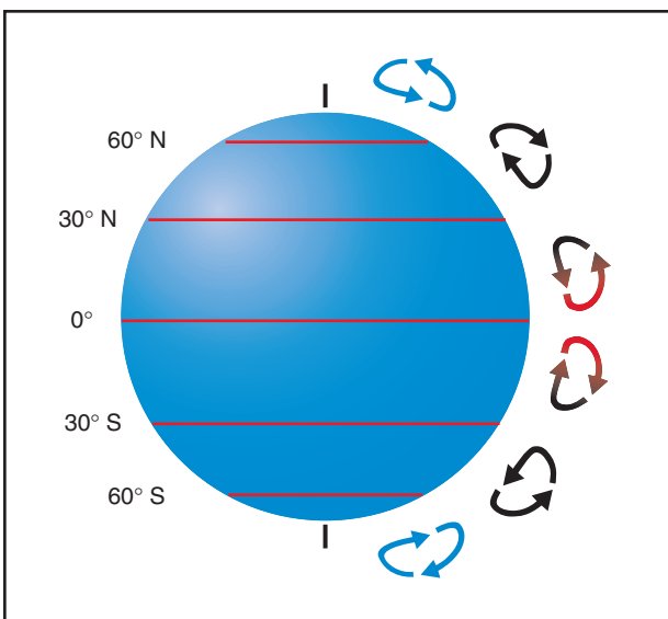
Figure 10-9. Three-cell circulation pattern due to the rotation of the Earth.
